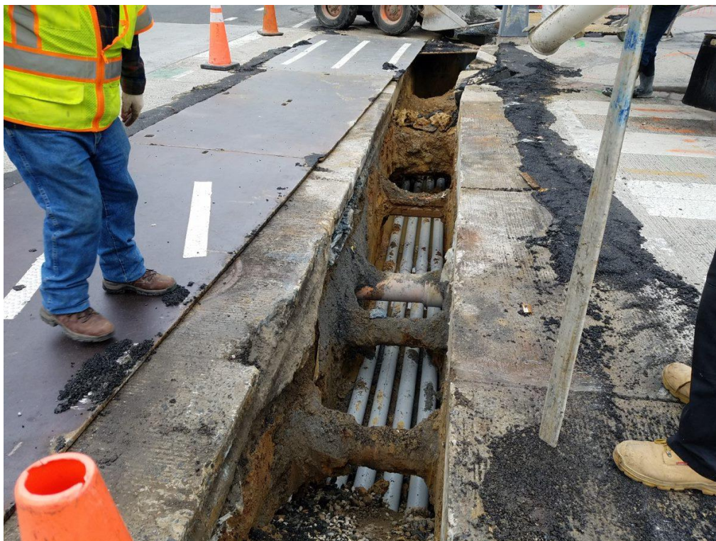
Installation of 4' PVC Conduit at the NE corner of V Street
